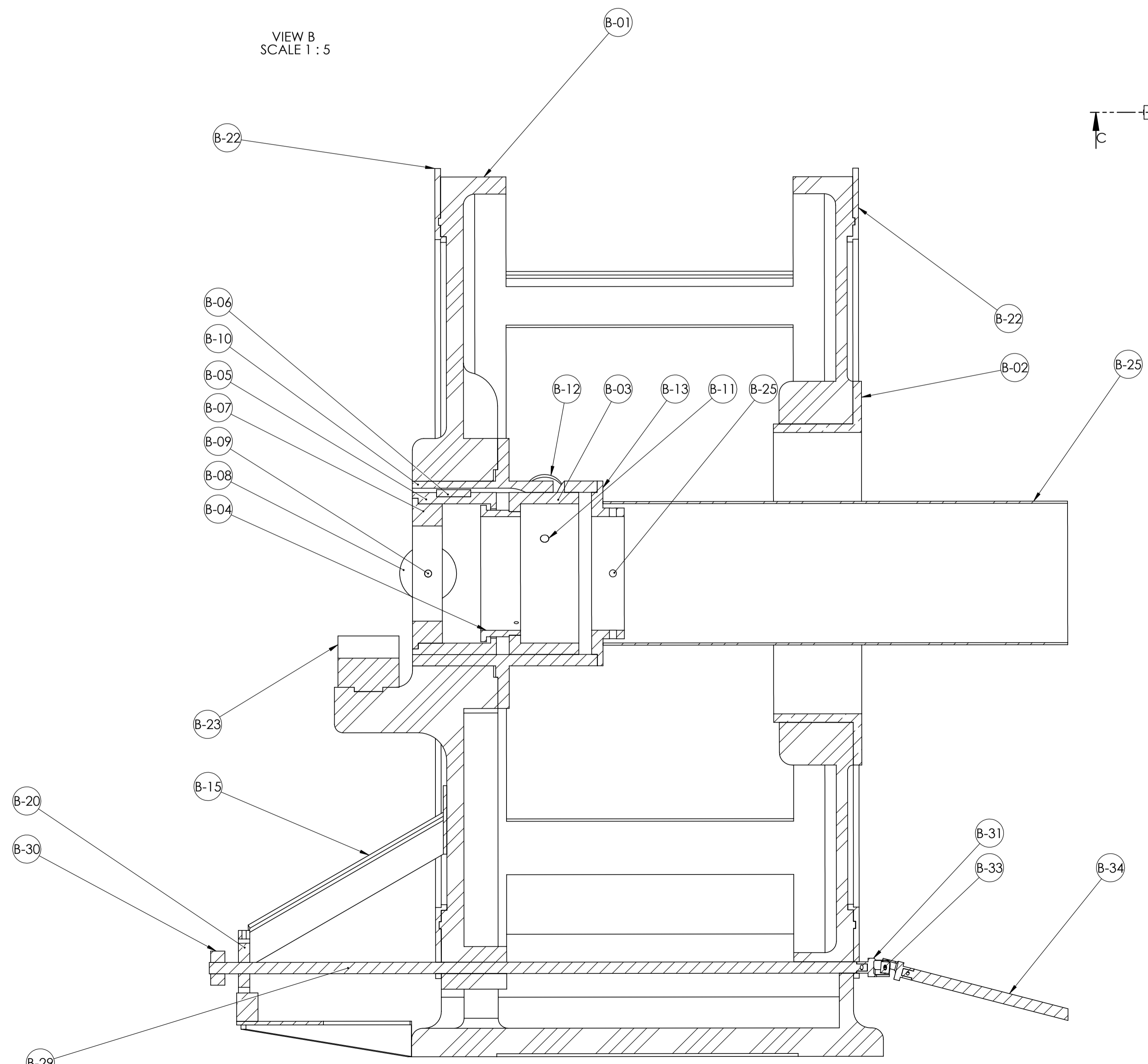
SECTION C-C SCALE 1 : 2
