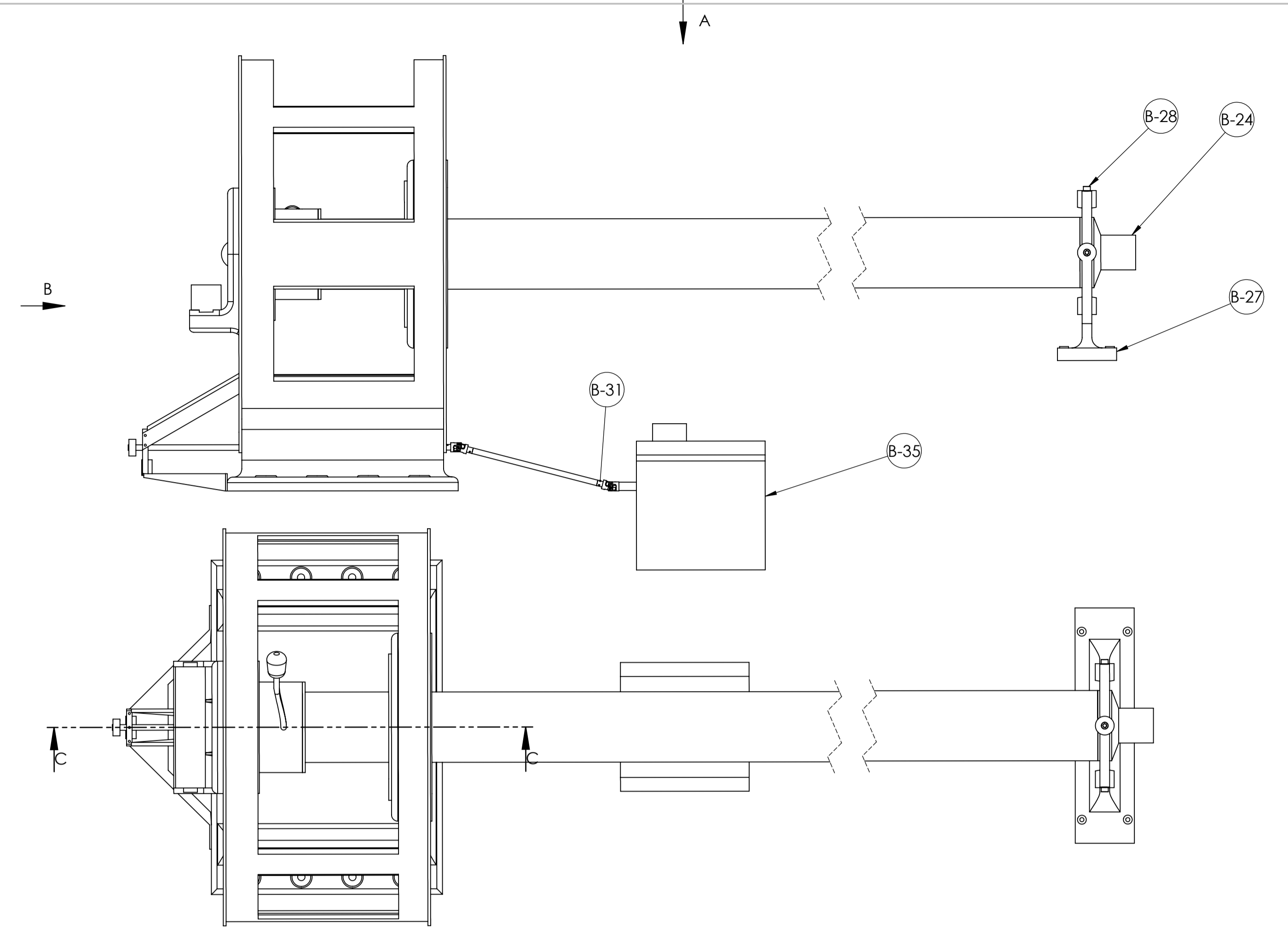
VIEW A SCALE 1 : 5
